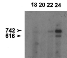
Figure 7 Radioactively labeled PCR amplification of cDNA from IV-8, by use of primer pair 3/2. Four identical samples were amplified, for 18, 20, 22, or 24 cycles; the number of cycles is indicated above the appropriate lane. The autoradiograph shows progressive accumulation of product for both the mutant (616 bp) and normal (742 bp) alleles, with no evidence of any additional bands. The film was analyzed by densitometry, to estimate the relative amounts of each transcript. Analysis of cDNA from patient IV-9 gave comparable results (data not shown).
